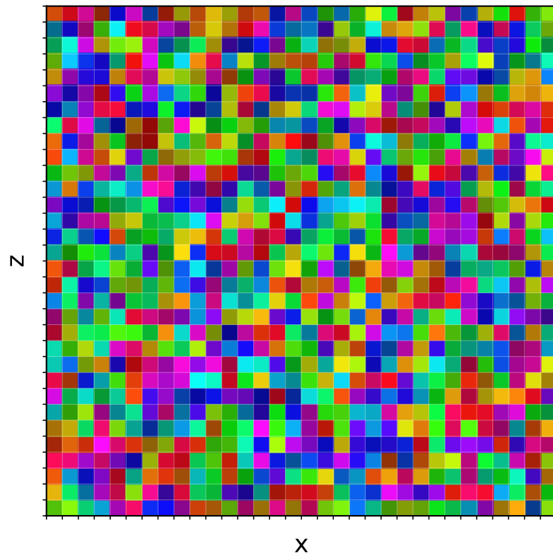
High T = 2.10: disordered
