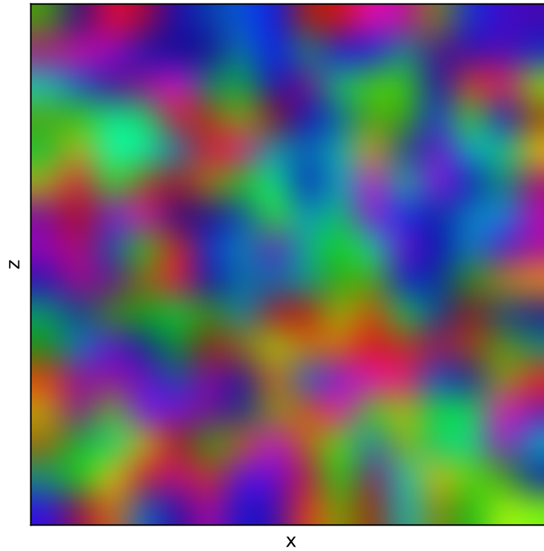
High T: disordered
