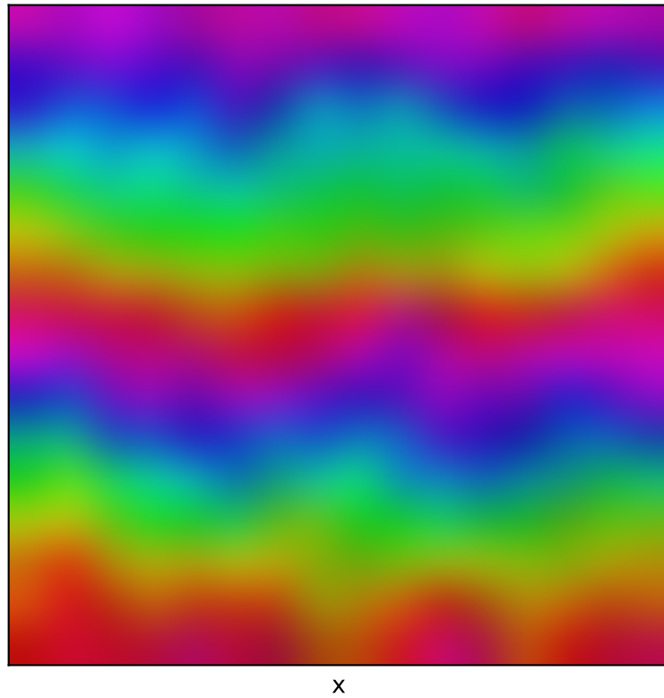
Low T: helical
