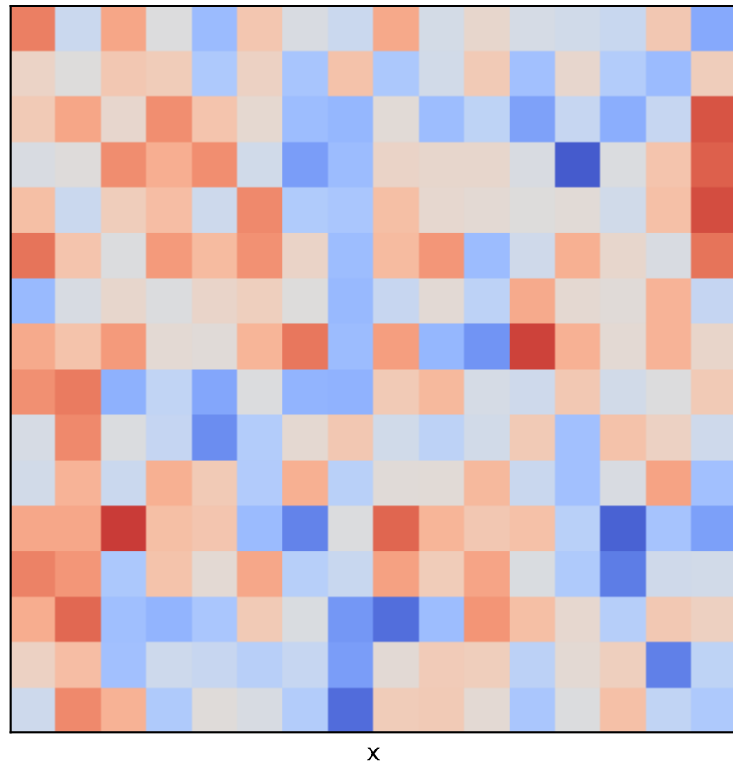
Low T: S_z
