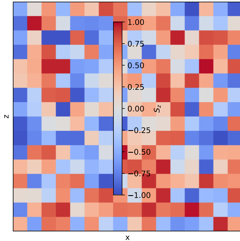
High T: S_z
