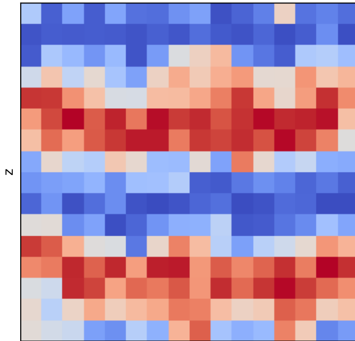
Low T spin components
