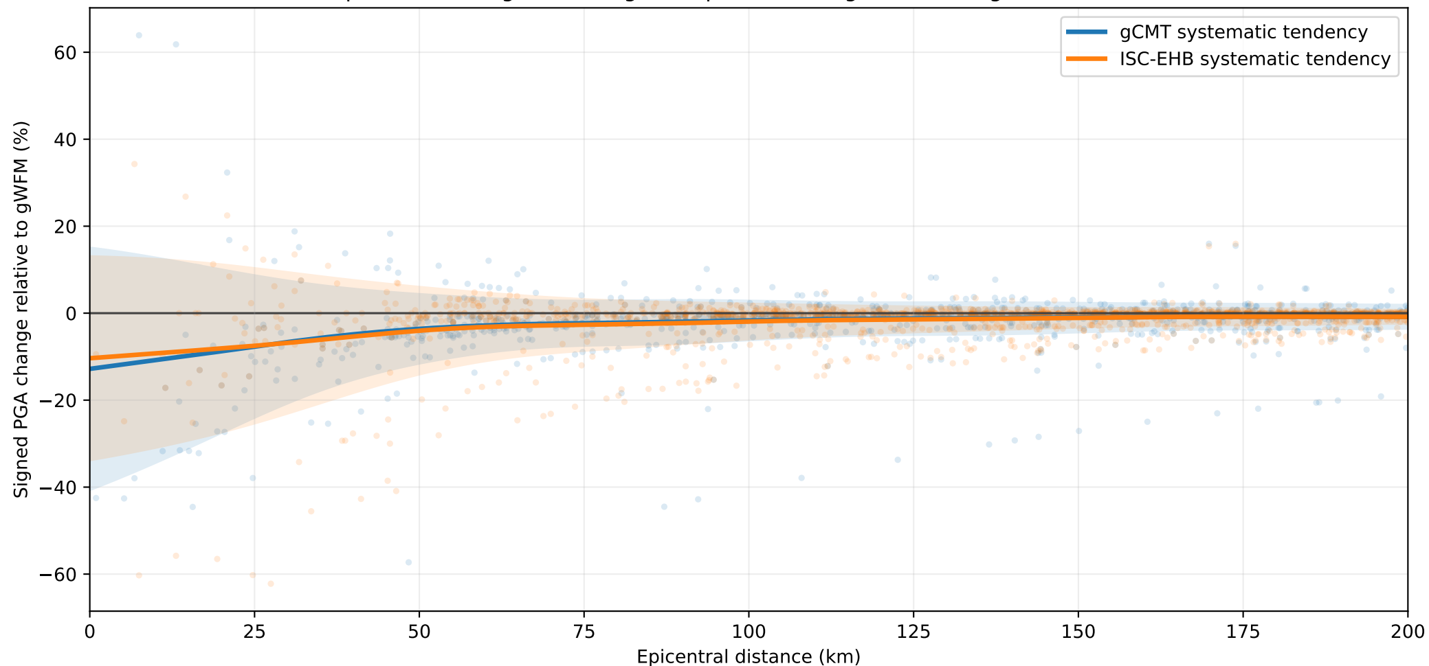
Signed PGA sensitivity to catalogue depth Comparison catalogue minus gWFM: positive = higher PGA; negative = lower PGA
