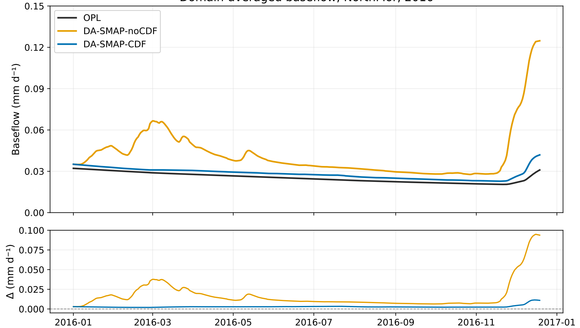
Domain-averaged baseflow, NorthMor, 2016
