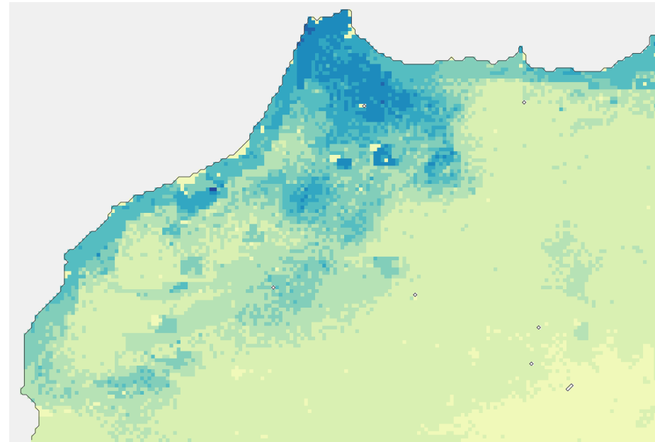
(b) DA-SMAP-noCDF
