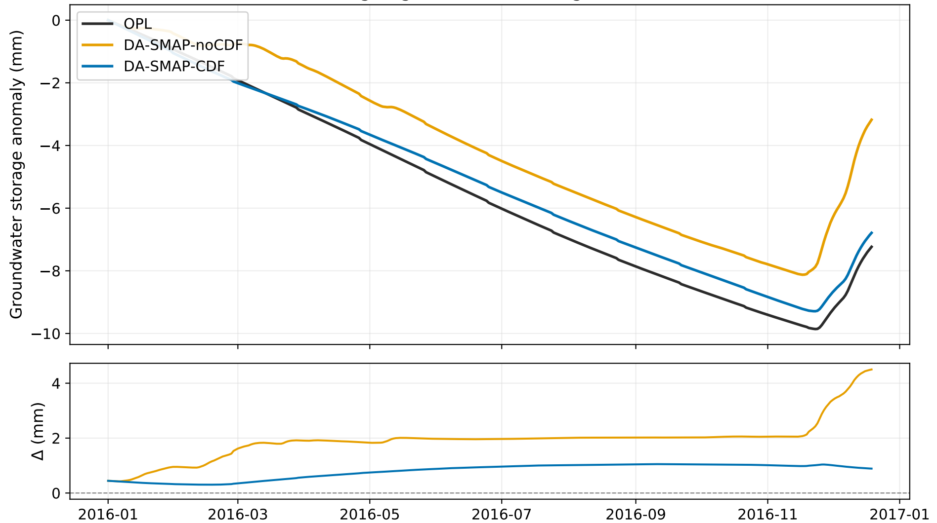
Domain-averaged groundwater storage, NorthMor, 2016
