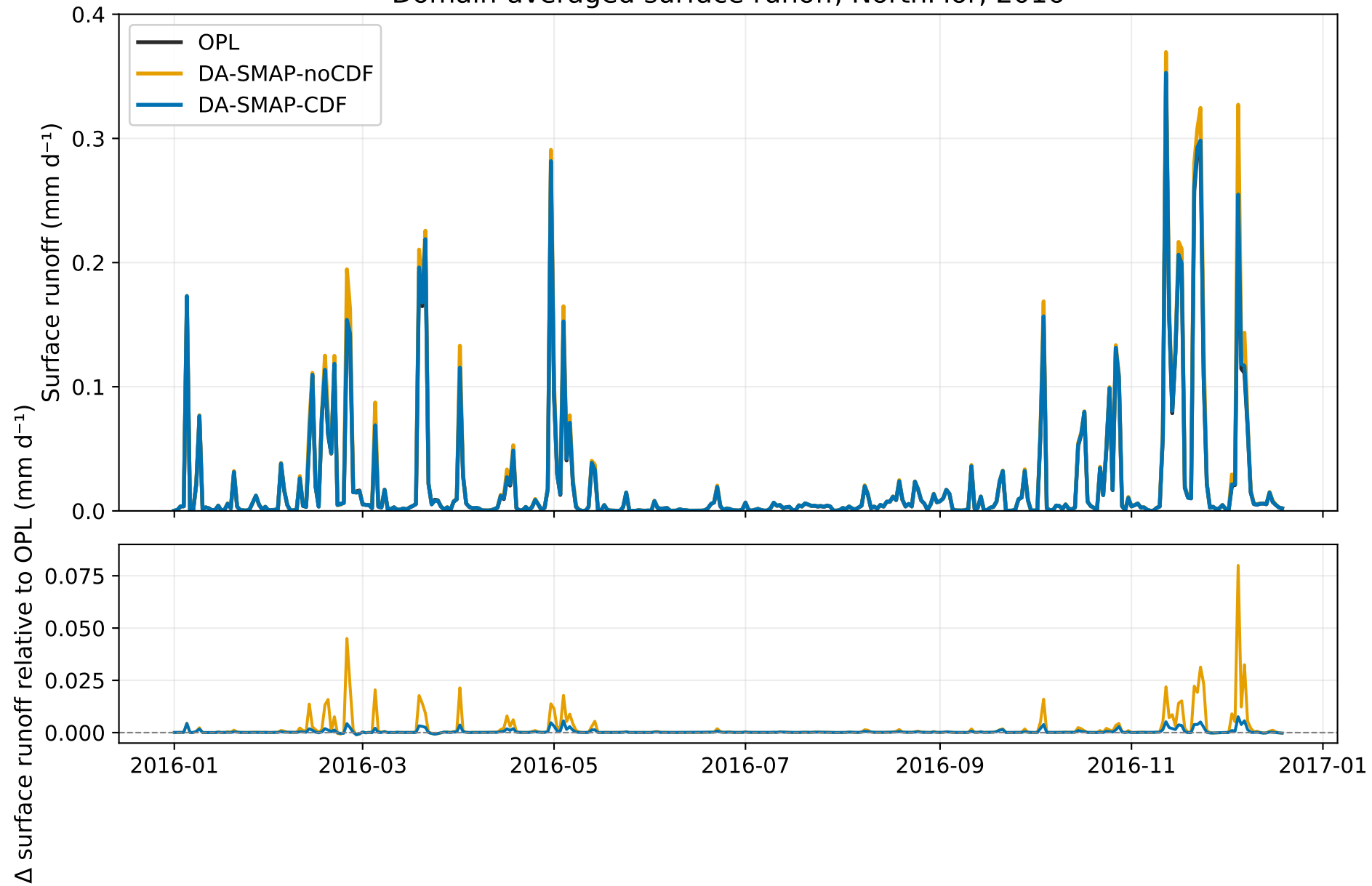
Domain-averaged surface runoff, NorthMor, 2016
