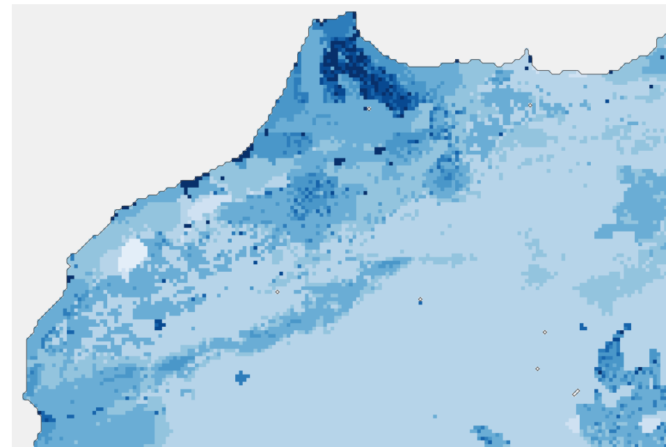
(b) DA-SMAP-noCDF
