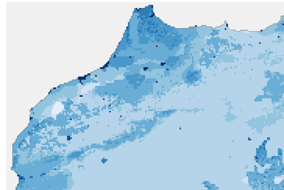
(c) DA-SMAP-CDF
