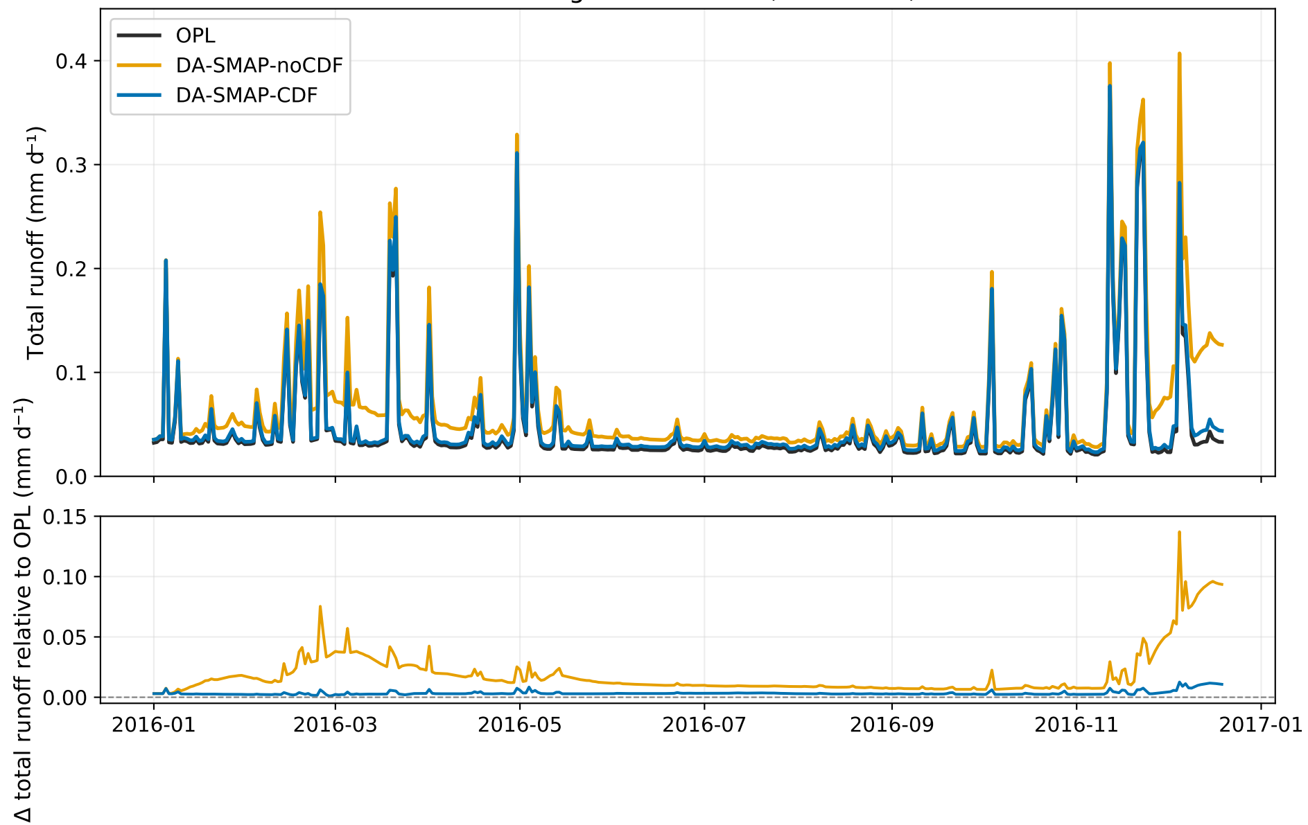
Domain-averaged total runoff, NorthMor, 2016
