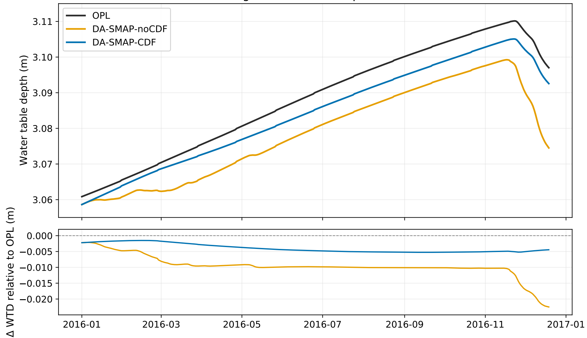
Domain-averaged water table depth, NorthMor, 2016
