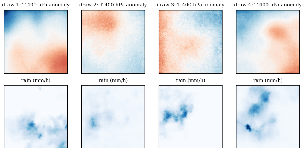
Figure 10. Four unconditional samples from the diffusion prior after 60,000 training steps: 400 hPa temperature anomaly from the domain mean (top) and rain rate (bottom), 128 \times 128 at 4 km.
