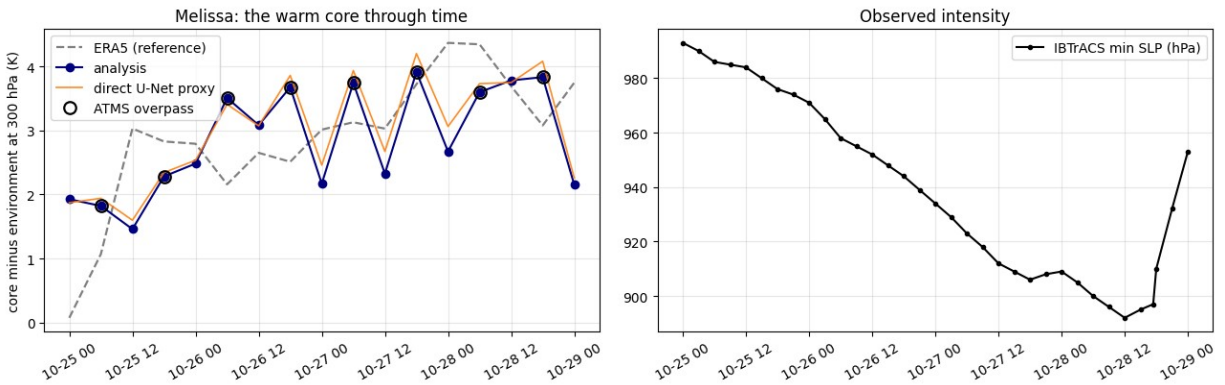
Figure 16. Melissa: the 300 hPa warm core through the storm for ERA5, the 8-member analysis and the direct U-Net proxy, with ATMS overpasses marked, and the observed minimum pressure from IBTrACS.
