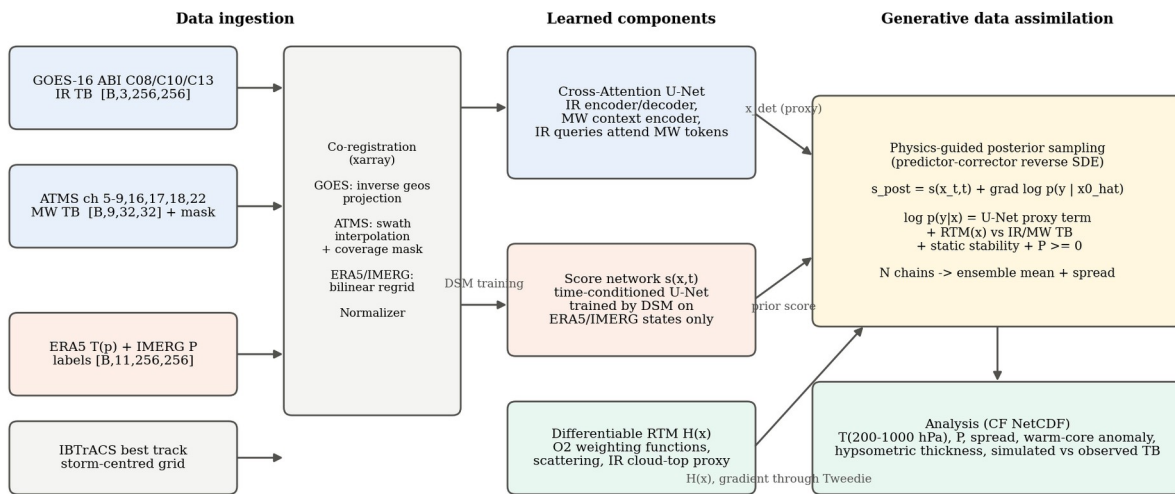
Figure 1. End-to-end architecture of vaughan. Blue boxes carry observations, orange boxes carry the learned state prior and its labels, green boxes are physics operators and outputs, and the yellow box is the generative data-assimilation step.
