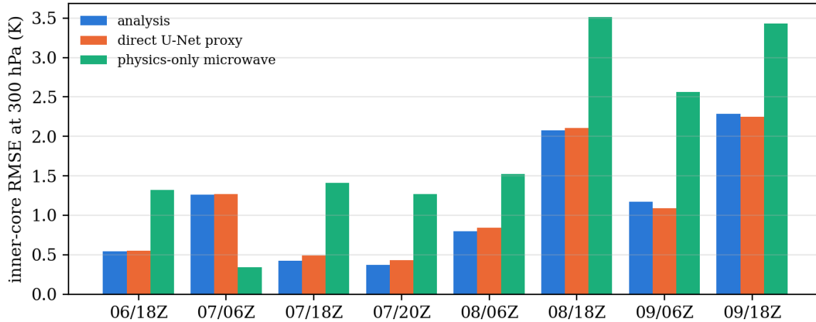
Figure 9. Inner-core temperature RMSE at 300 hPa (central 16 x 16 pixels, about 70 km) against ERA5 on the eight scenes with an ATMS overpass, for the full analysis, the direct U-Net proxy alone, and the physics-only microwave retrieval.
