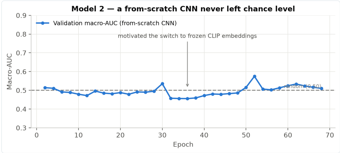
Figure 2. The from-scratch convolutional tissue classifier never left chance level (validation macro-AUC ≈ 0.50 across 68 epochs) — the result that motivated the switch to frozen CLIP embeddings.
