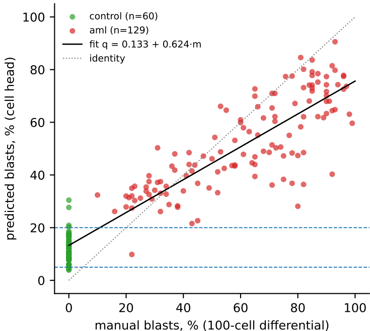
AML-MLL, 189 patients: offset + scatter ( \phi = 9.2 / 24.8 )
