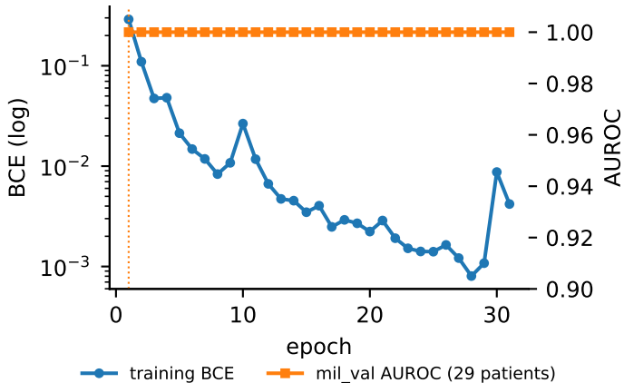
MIL head: AUROC saturated → epoch 1 retained
