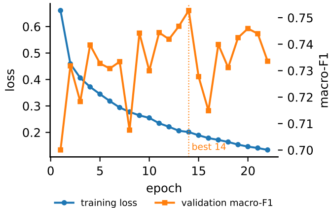
Cell head (early stop on macro-F1)
