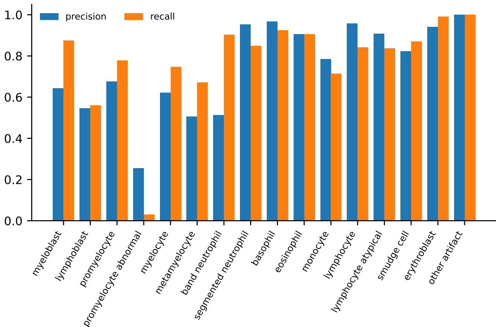
Cell head on definite-label validation cells (14 121; macro-F1 0.753)
