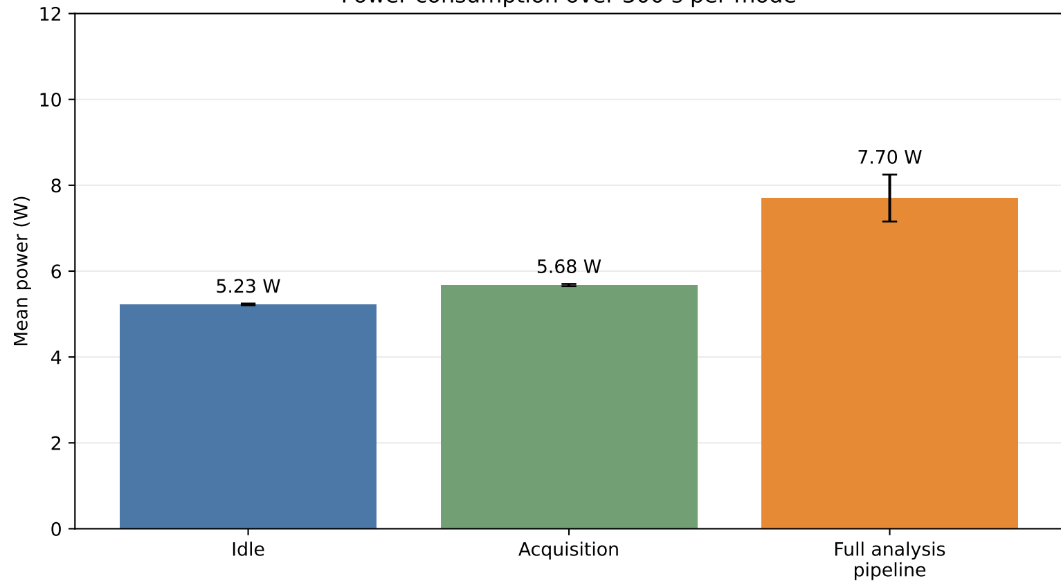
Power consumption over 300 s per mode
