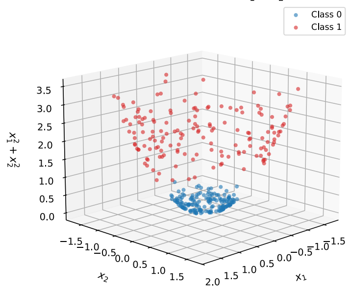
Feature space ( x_1, x_2, x_1^2 + x_2^2 )
