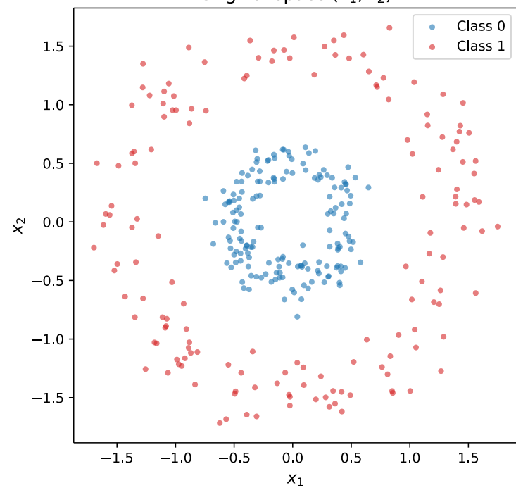
Original space ( x_1, x_2 )
