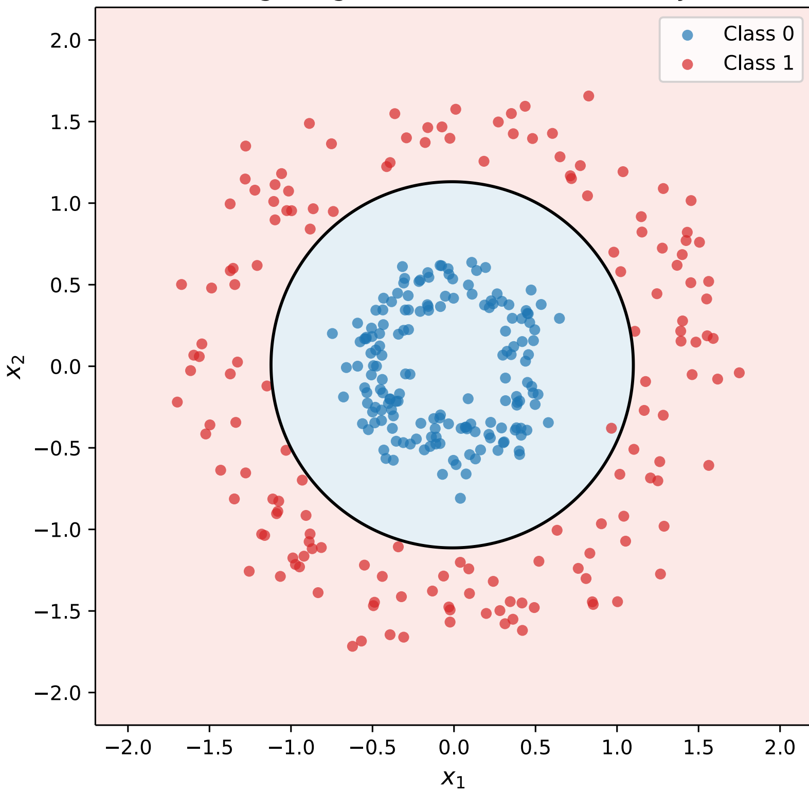
Ridge Regression Decision Boundary
