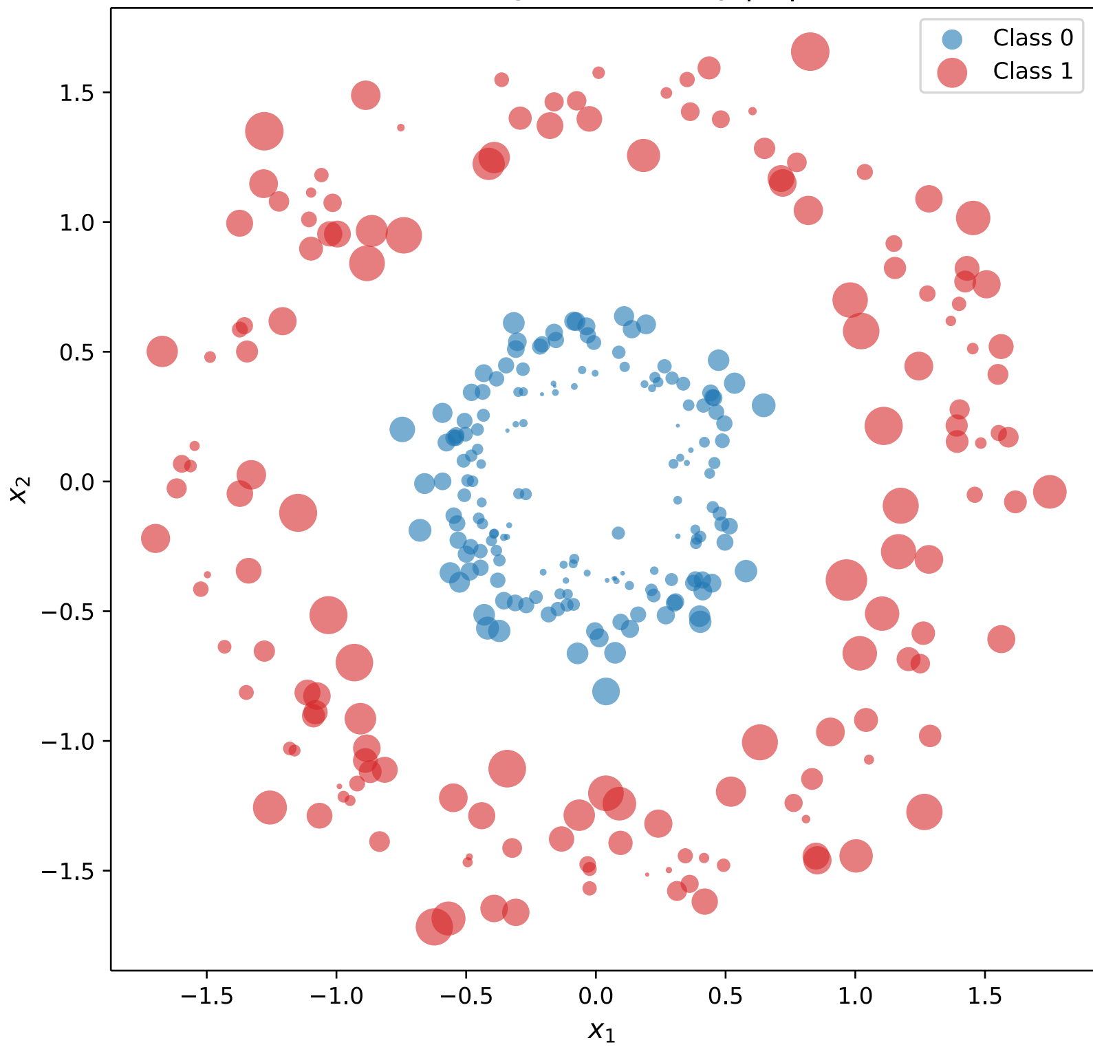
Training data sized by |\alpha_n|
