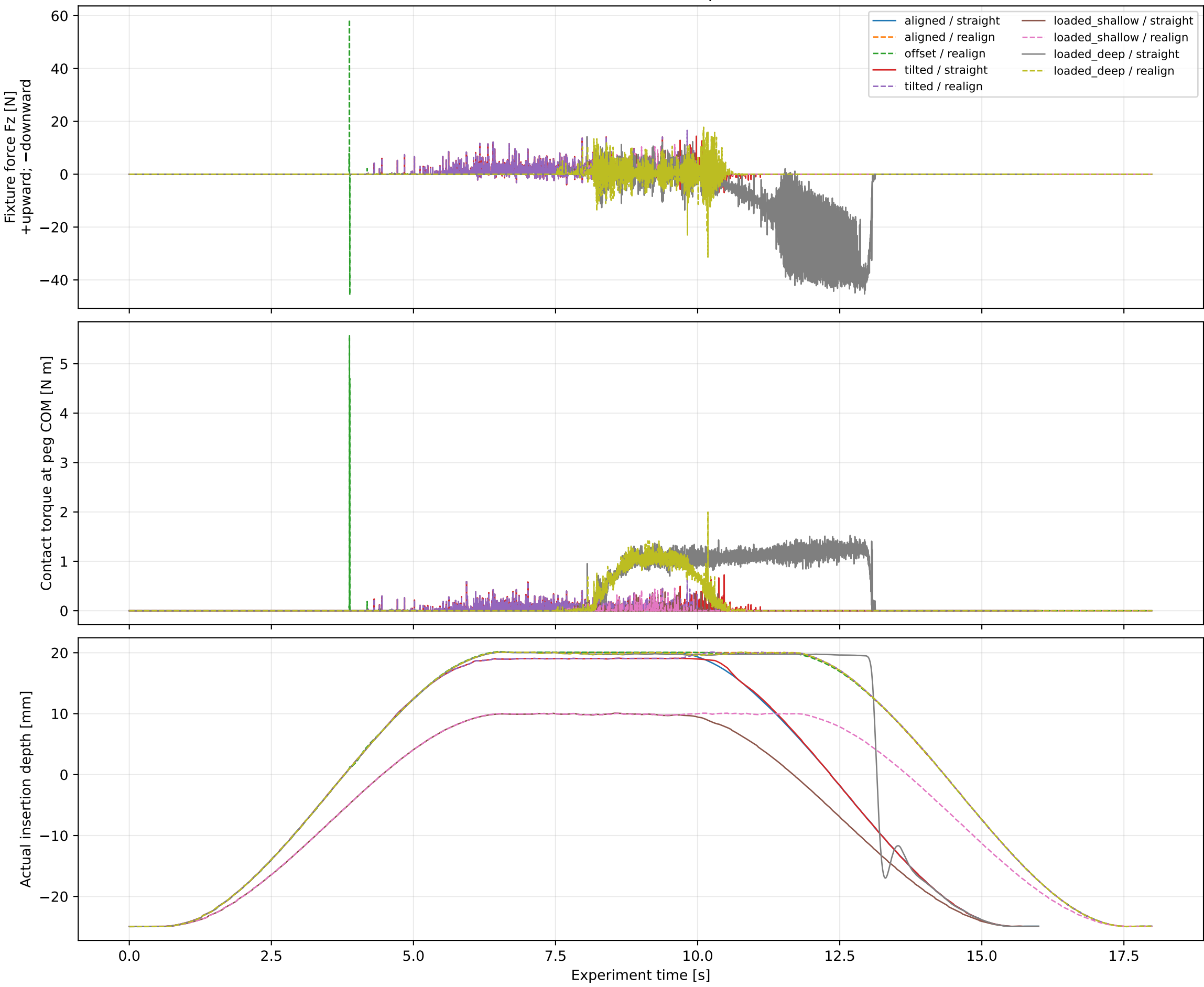
FR3 simulation: full contact force, torque and actual motion
