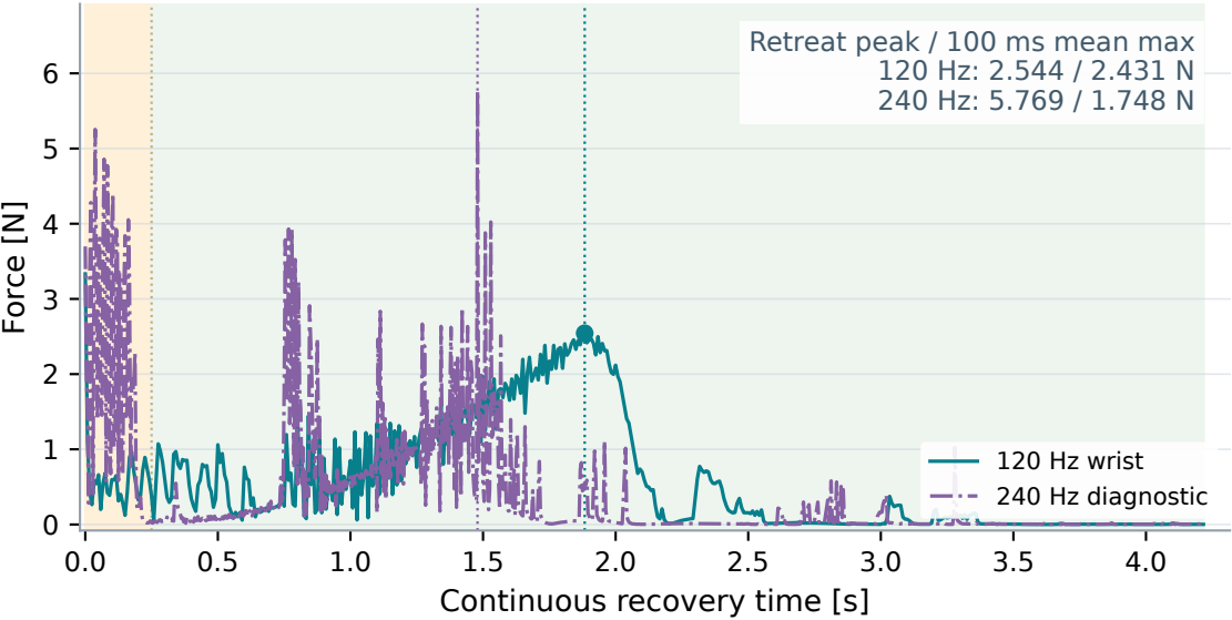
Raw wrist force: peak and sustained load differ
