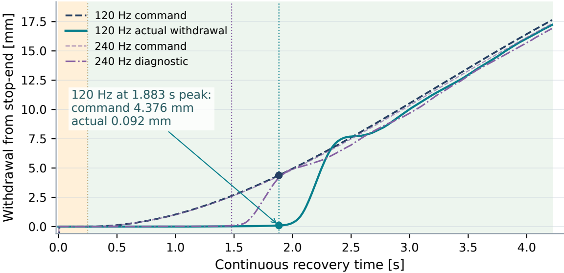
Commanded and actual withdrawal in each run
