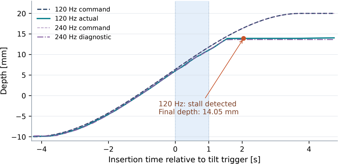
Independent insertion trajectories
