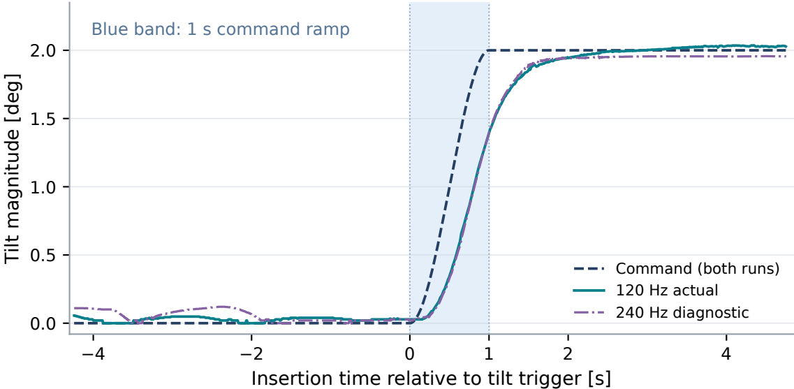
Actual tilt under the same nominal command
