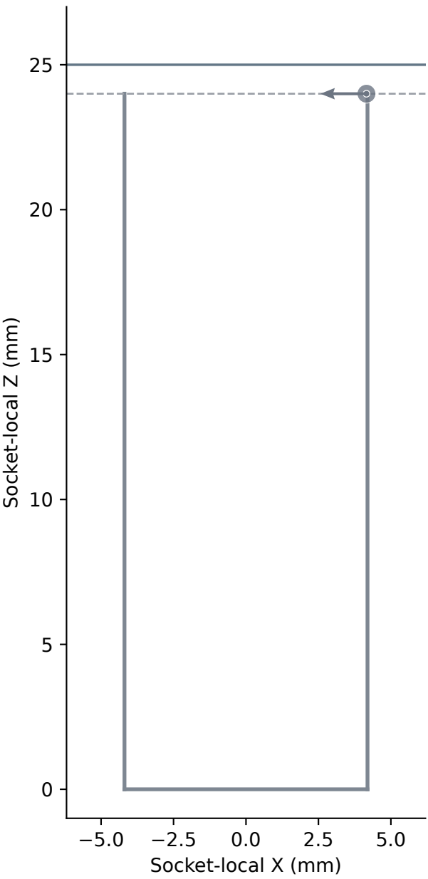
Reference contact locations max \Sigma N = 2.590 N at 9.042 s
