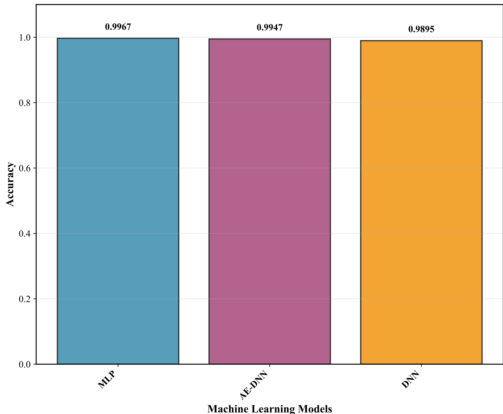
MODEL ACCURACY COMPARISON
