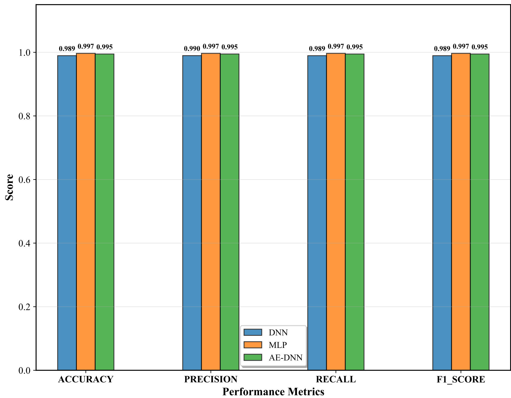
DETAILED PERFORMANCE METRICS COMPARISON
