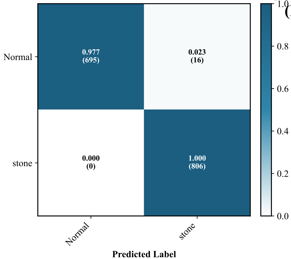
DNN Confusion Matrix
