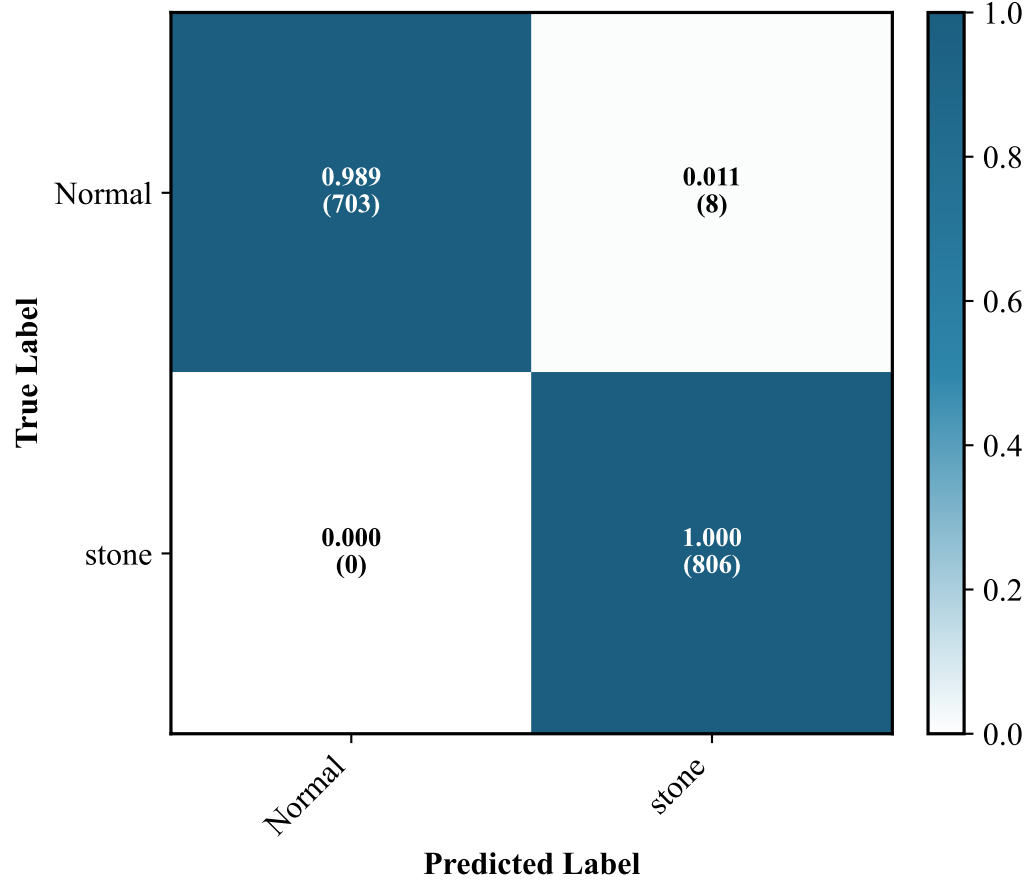
AE-DNN Confusion Matrix
