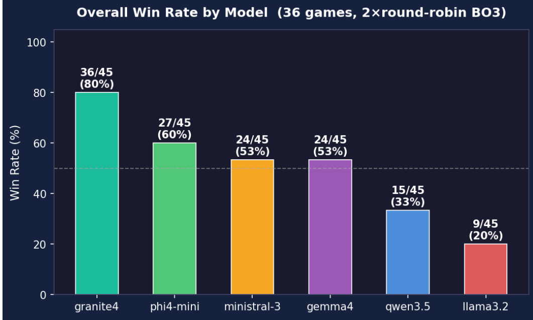
Figure 1: Overall win rates by model (bar chart).
