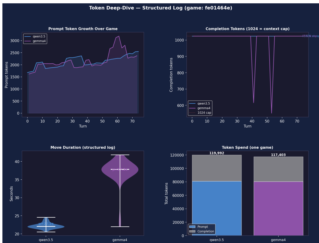
Figure 9: Four-panel deep dive: prompt tokens, completion tokens, move duration, and cumulative token spend by model.
