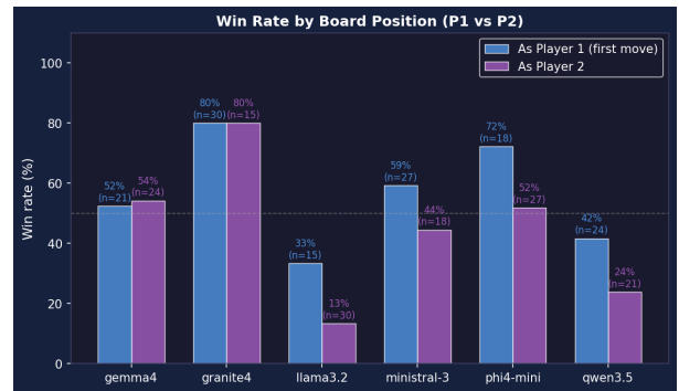
(b) Win rate as P1 vs. P2 per model.
