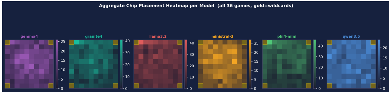
Figure 10: Board heatmaps: chip placement density per model on the 10 \times 10 grid.
