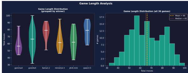
(a) Game length distribution by outcome.
