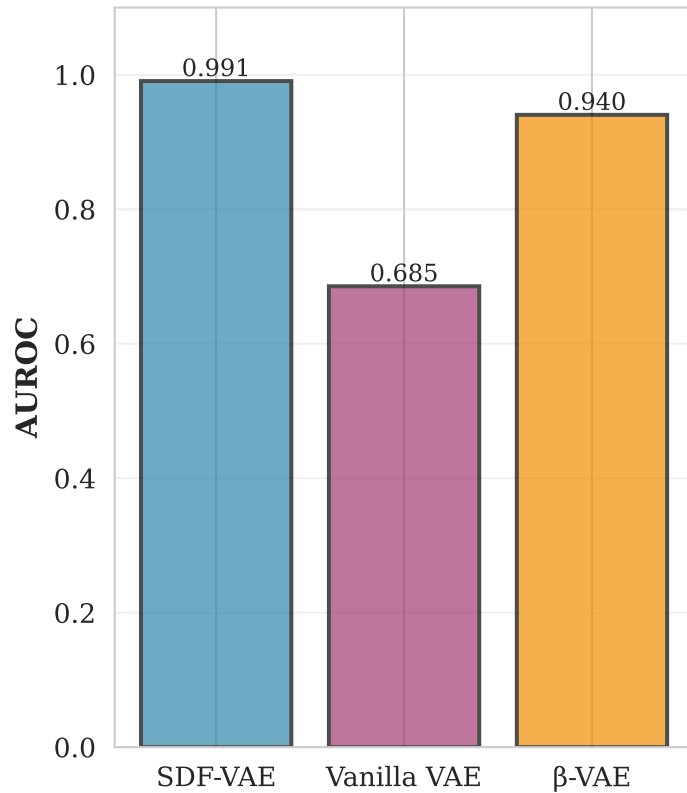
(b) OOD Detection (Recon. Error)
