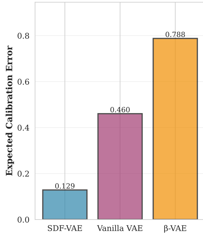
(a) Uncertainty Calibration
