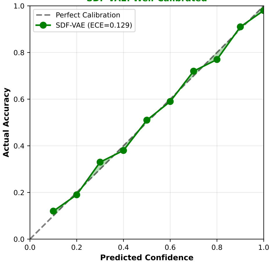
SDF-VAE: Well-Calibrated
