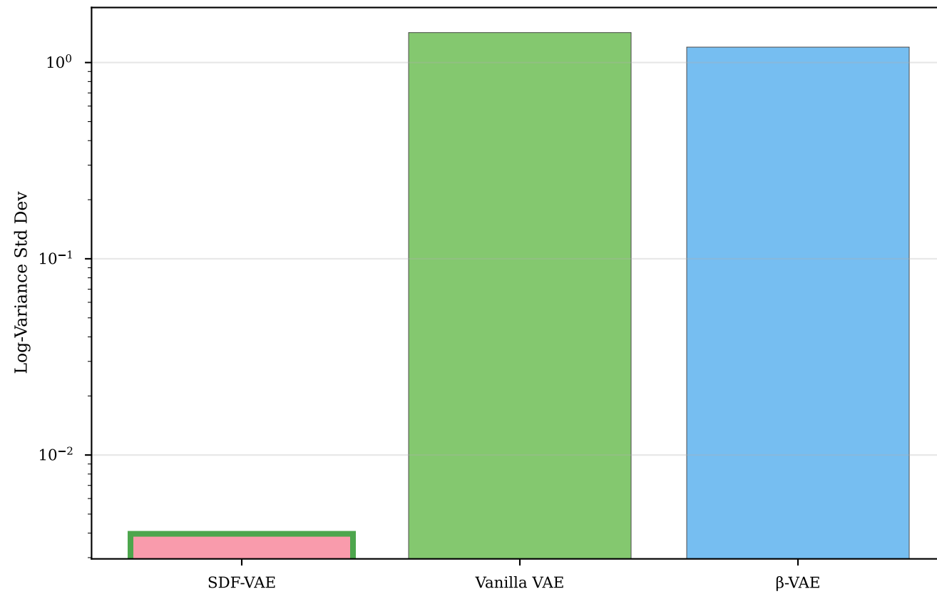
Latent Variance Stability Lower is More Stable
