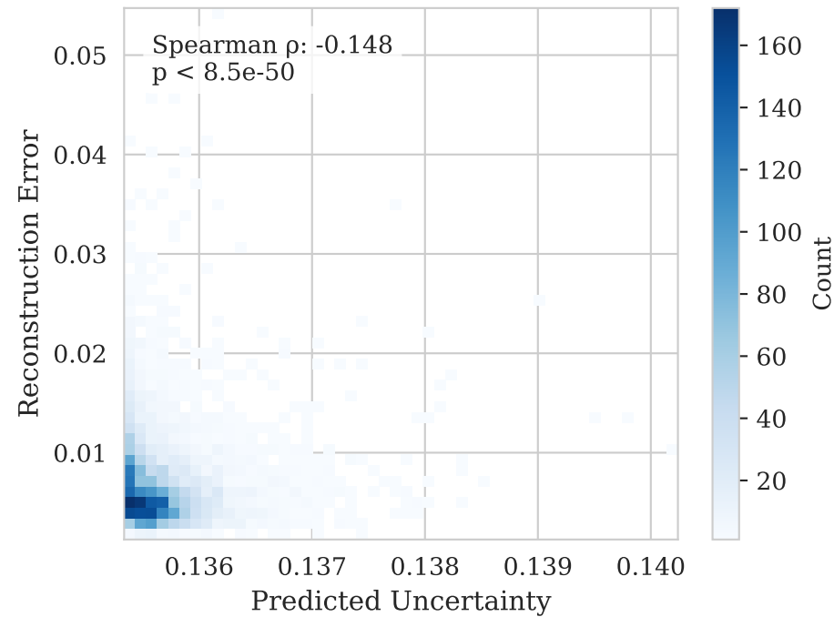
SDF-VAE
