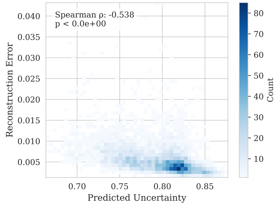
\beta -VAE
