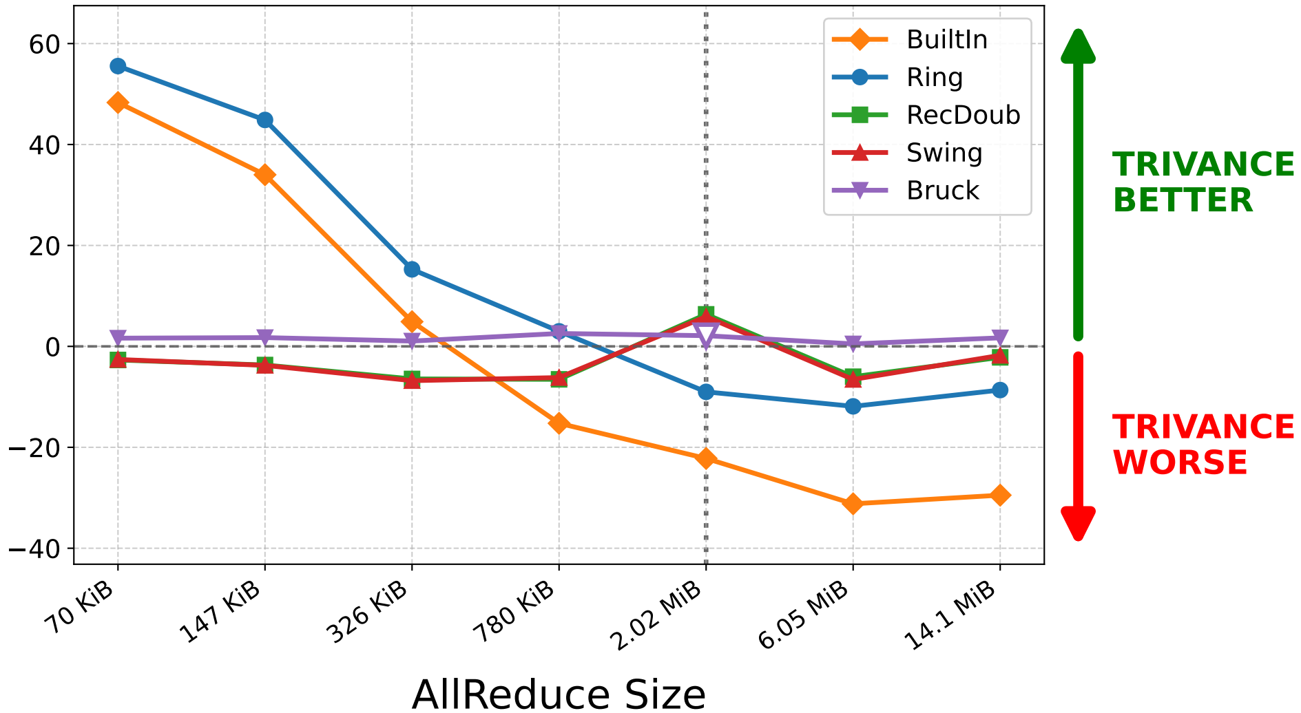
Relative Completion Time vs. Trivance (%)
