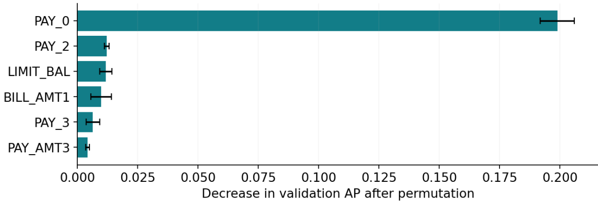
Figure 4. Tuned XGBoost validation permutation importance, top six features. Error bars are the SD across five permutations, not confidence intervals or causal estimates. Horizontal units: decrease in validation AP.
