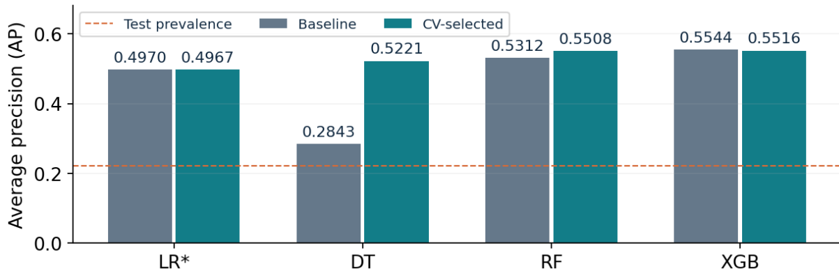
Figure 2. Test AP for declared baselines and CV-selected models. The dashed reference is positive prevalence (0.2212). Selection uses fit-fold CV, never this chart.
