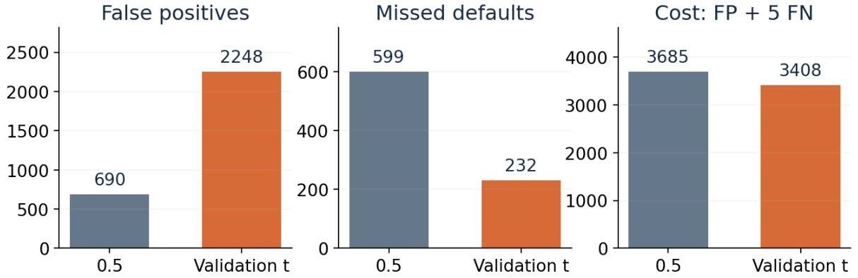
Figure 3. Moving the same tuned XGBoost from 0.5 to its validation cutoff changes FP/FN and workload. Ranking scores remain unchanged.
