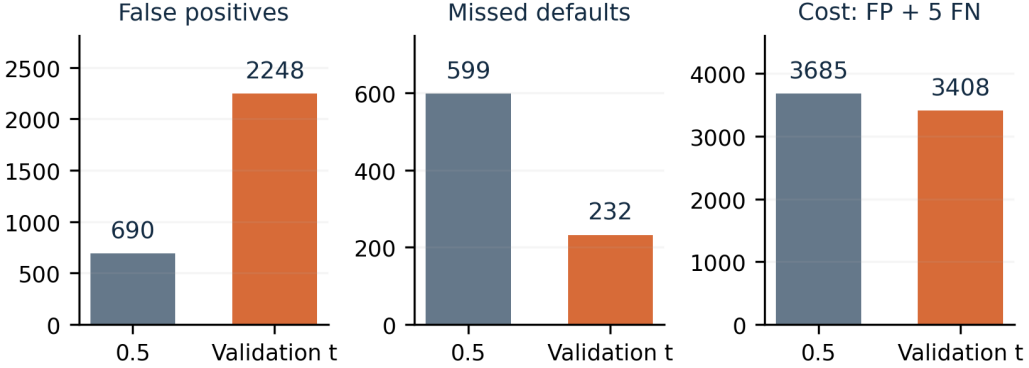
Figure 2: Moving the same tuned XGBoost from 0.5 to its validation cutoff changes FP/FN and workload. Ranking scores remain unchanged.
