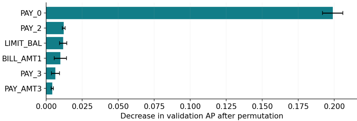
Figure 3. Tuned XGBoost validation permutation importance, top six features. Error bars are the SD across five permutations, not confidence intervals or causal estimates. Horizontal units: decrease in validation AP.
