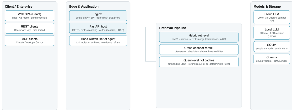
Figure 1: DocMind deployment and data flow. Enhancements (reranker, caches, web search) degrade gracefully; the answering path never depends on them succeeding.
