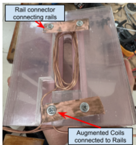
Figure A7: Close-up of Acrylic Housing
