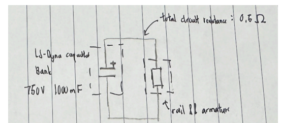
Figure 4: Simulation's Mass-Driver RC Circuit
