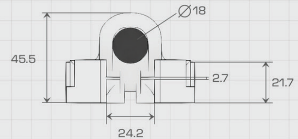
Rear View
