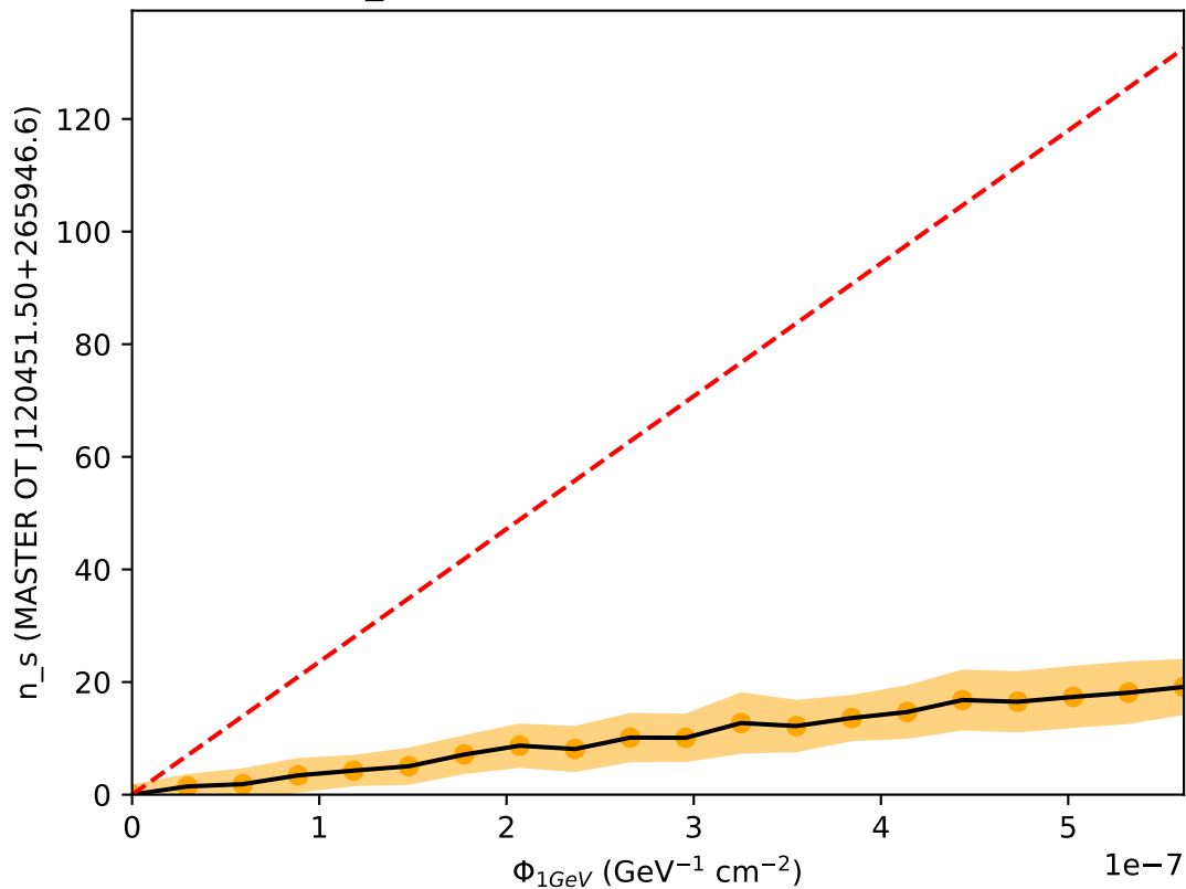
Bias ( n_s (MASTER OT J120451.50+265946.6))
