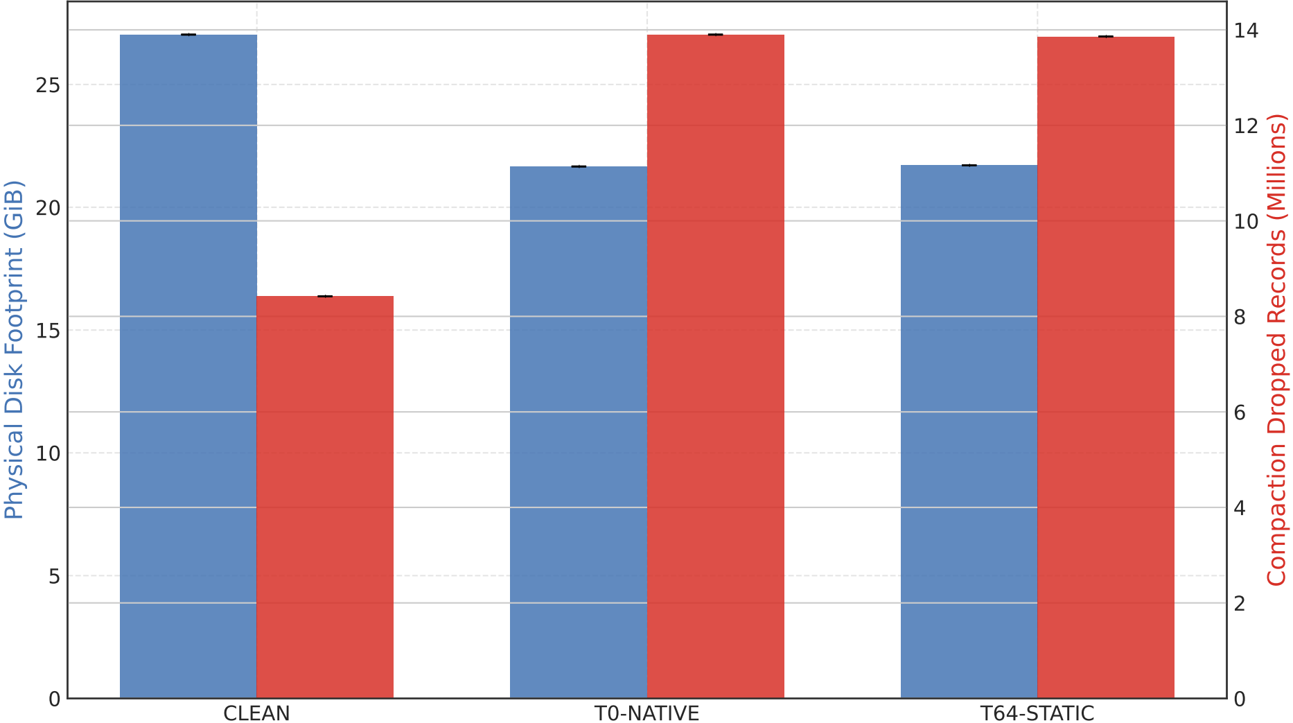
Post-Workload Debt Convergence: Physical Footprint vs Tombstone Cleanup
