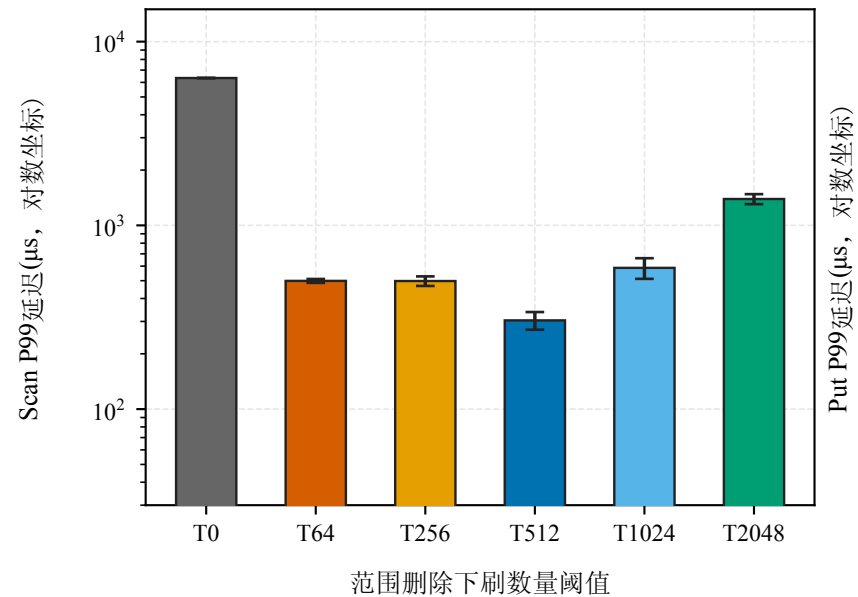
(a) Scan P99读取尾延迟
