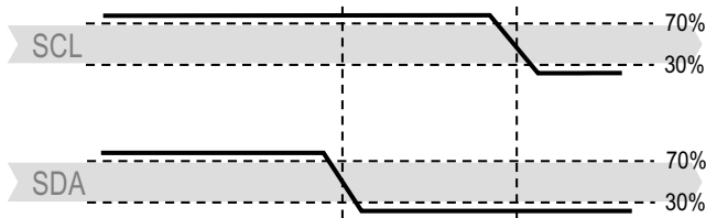
Figure18 Start Transmit State (S) - When SCL is at high level, SDA is converted from high level to low level. The start state is a special bus state controlled by the main engine, indicating the start of slave machinetransit (after Start, BUS is generally considered to be in a busy state).
