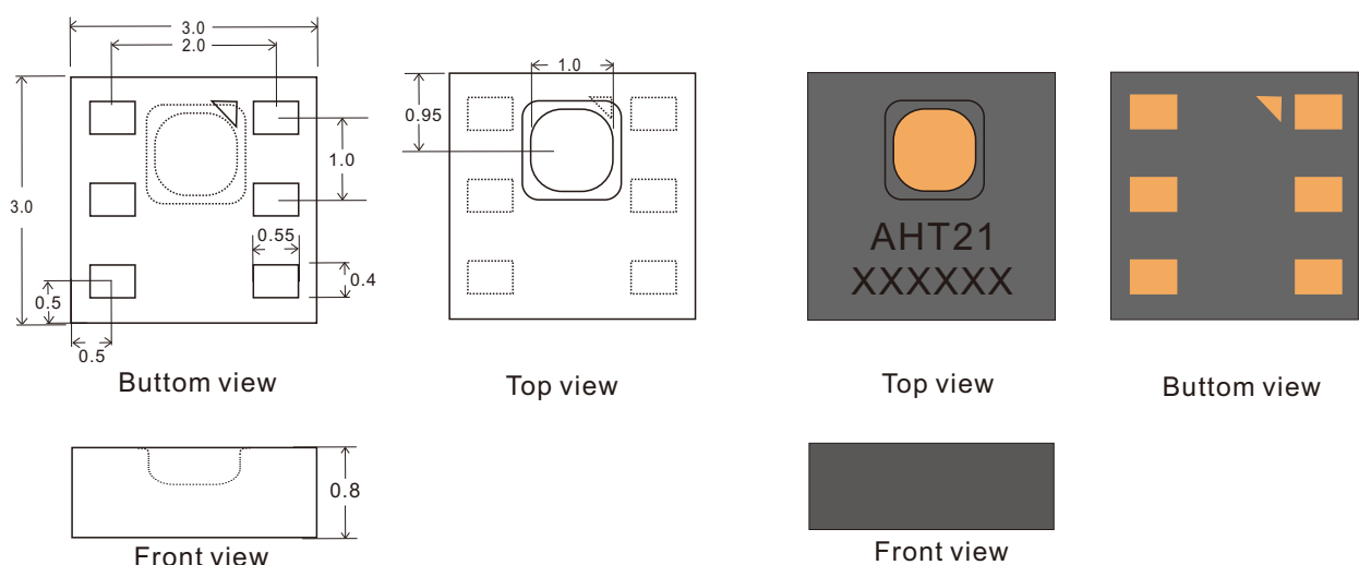
Figure 1: AHT21 Sensor Package Diagram (Unit: mm Tolerance: \pm 0.1 mm)
