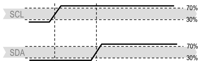
Figure19 Stop Transmit State (P) - When the SCL is at high level, the SDA line is converted from low level to high level. Stop state is a special bus state controlled by the main engine, indicating the end of slave machine transmit (after Stop, BUS is generally considered to be in idle state).
