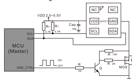
Figure 15-2 Typical application circuit 2, AHT21 operation is controlled by whether GND is grounded.
