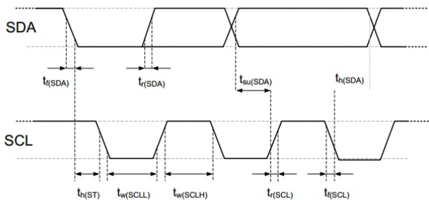
Figure 17 The figure sequence diagrams and abbreviations of digital input/output are explained in Table 8. Thicker SDA lines are controlled by sensors, and ordinary SDA lines are controlled by single chip computer. Please be noted that the effective read time of SDA is triggered by the drop edge of the previous conversion
