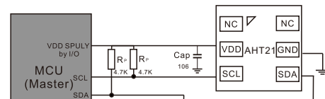
Figure 15-1 Typical application circuit 1, the pull-up voltage and VDD of SCL and SDA are powered by the MCU.
