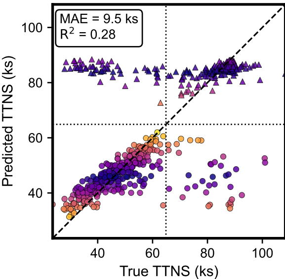
QRC Noiseless Simulation
