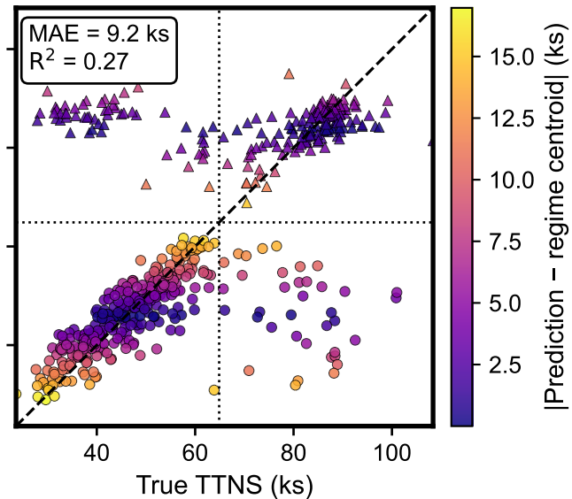
Classical XGBoost
