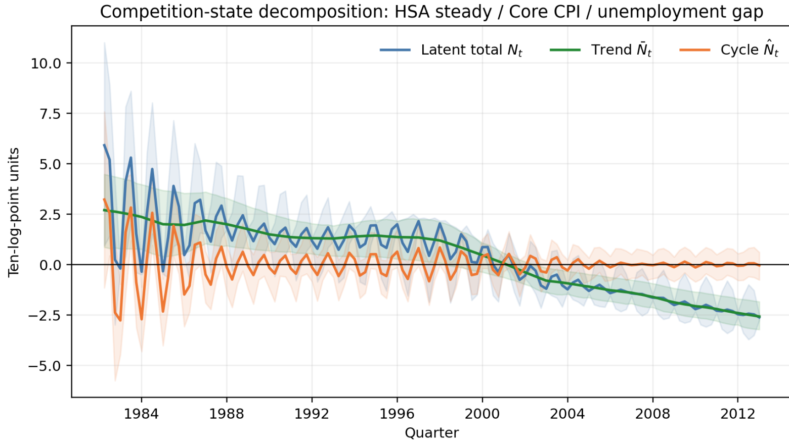
Figure 3: Posterior decomposition of the firm count N_t = \tilde{N}_t + \hat{N}_t under the main HSA steady (negative unemployment gap, core CPI), mixed-frequency design. Lines are posterior means, bands are 95% credible intervals. The quarterly states between the Q4 annual observations are inferred, not interpolated, so the bands widen between anchors.
