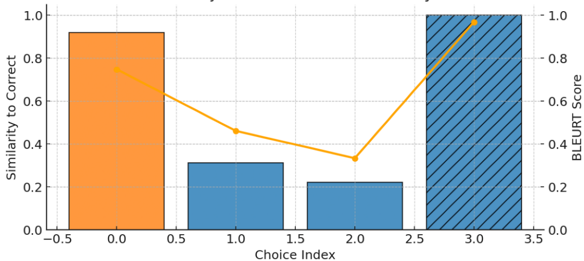
ReadIntBetween.json - Per-choice Similarity & BLEURT
