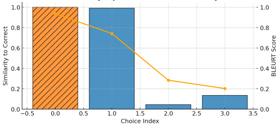
DeleteReservationByID.json – Per-choice Similarity & BLEURT
