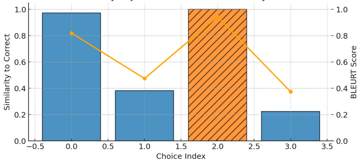
DeleteRoomByID.json - Per-choice Similarity & BLEURT
