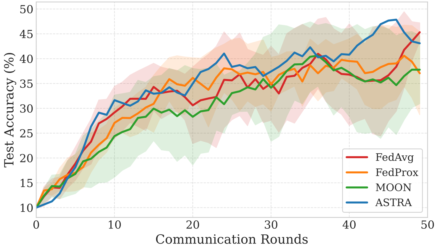
Convergence Comparison (Non-IID, \alpha = 0.1 )
