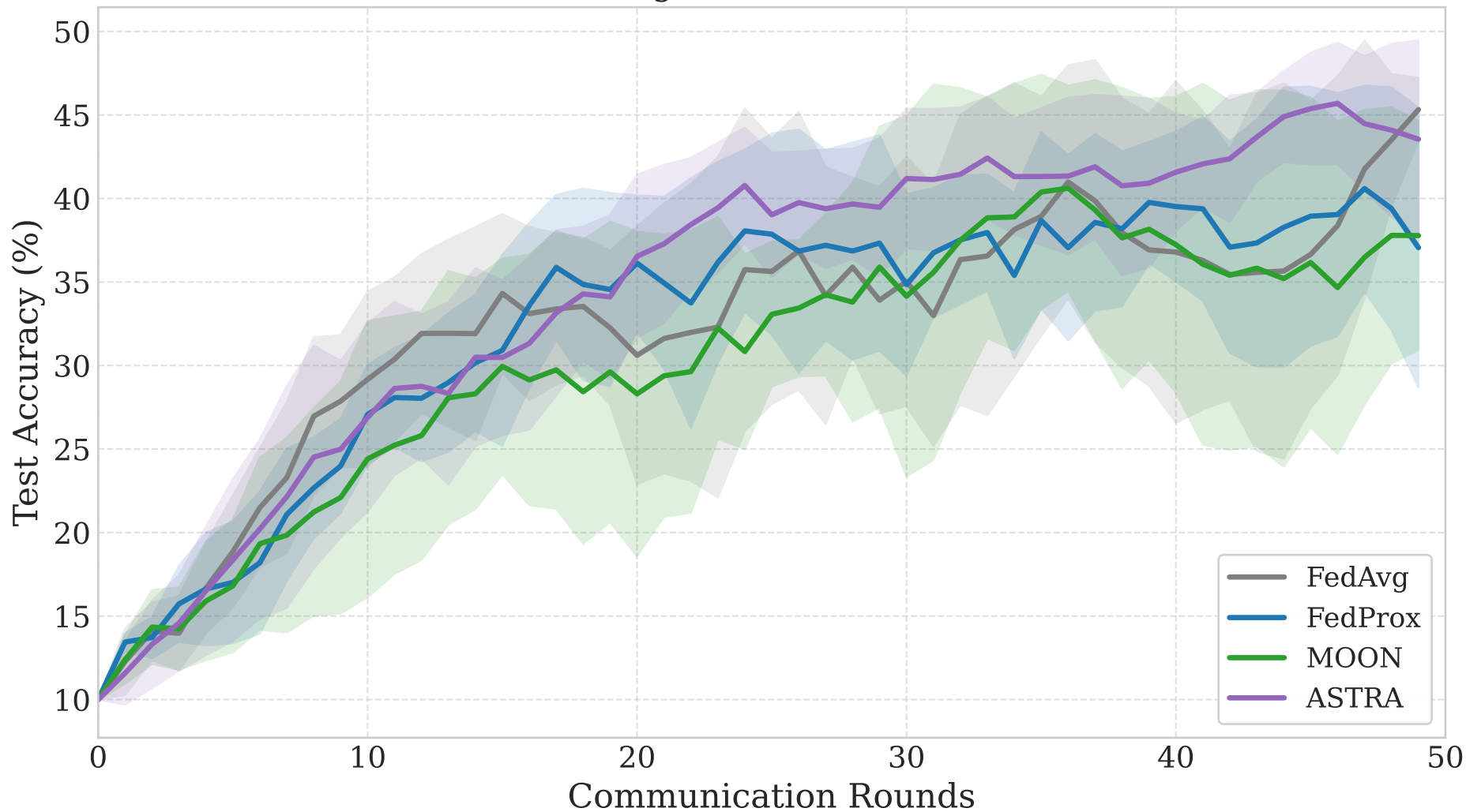
Non-IID Convergence (Smoothed Window=5)
