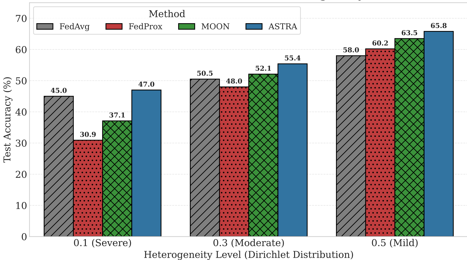
Model Robustness vs. Data Heterogeneity ( \alpha )
